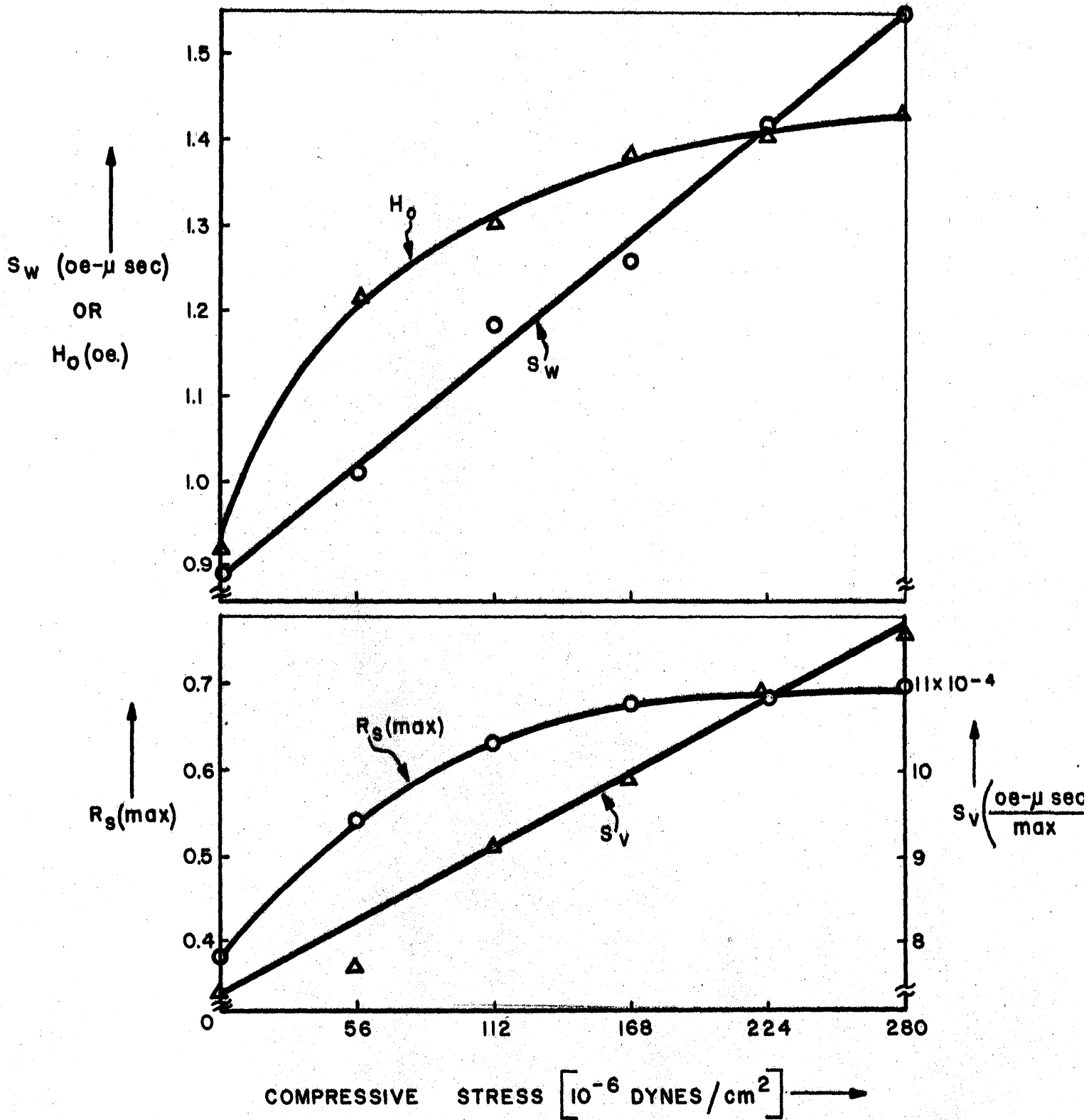
Fig. 6 Effect of compressive stress on several properties of a Ferroxcube-103 core (after N Menyuk (35)). The switching coefficient S_w and threshold field H_0 have been corrected for lack of loop squareness.
